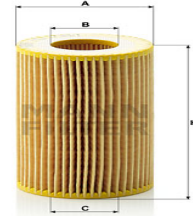
Oil Filter HU 718/1 k EM-10130
