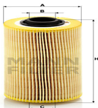
Oil Filter HU 938/1 x EM-10137
